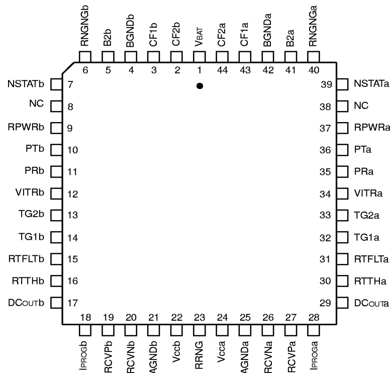
Figure 3. 44-Pin PLCC Pin Diagram
