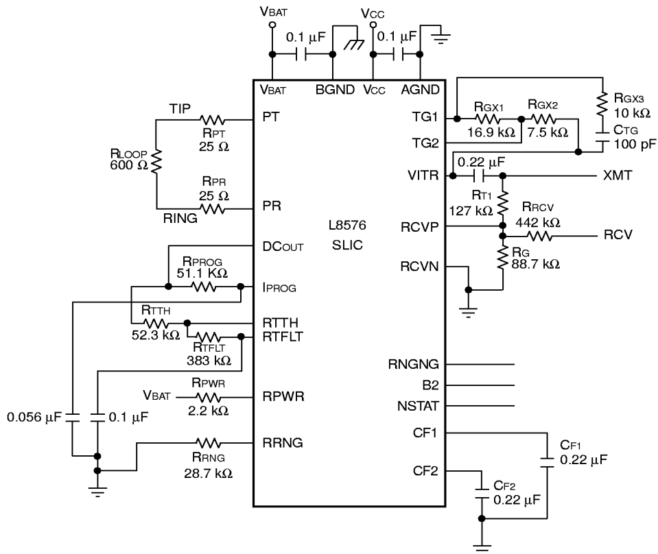
Figure 5. Basic Test Circuit
