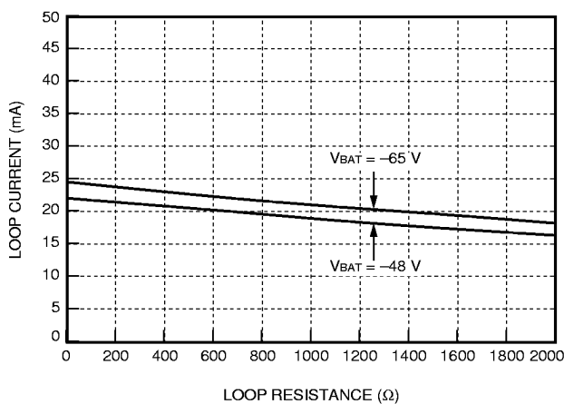
Figure 14. Loop Current vs. Loop Resistance
