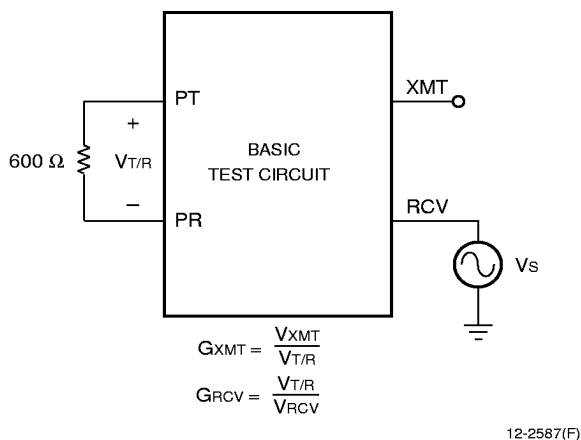
Figure 10. ac Gains
