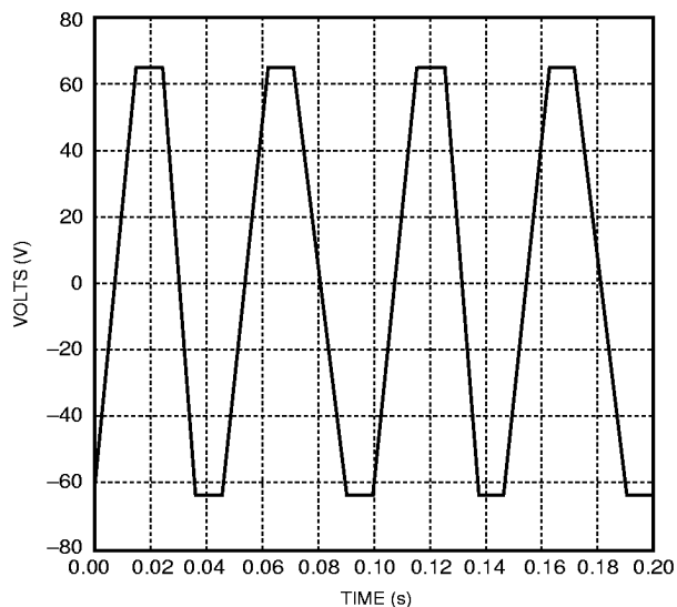
Figure 18. Ringing Waveform Crest Factor = 1.6
