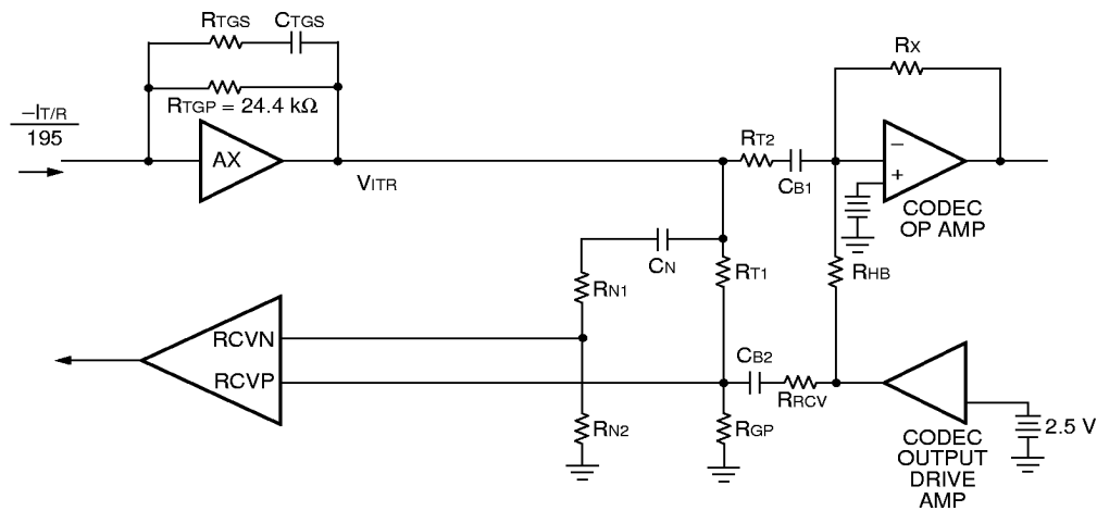
Figure 22. ac Interface Circuit Using First-Generation Codec (Including Blocking Capacitors)
