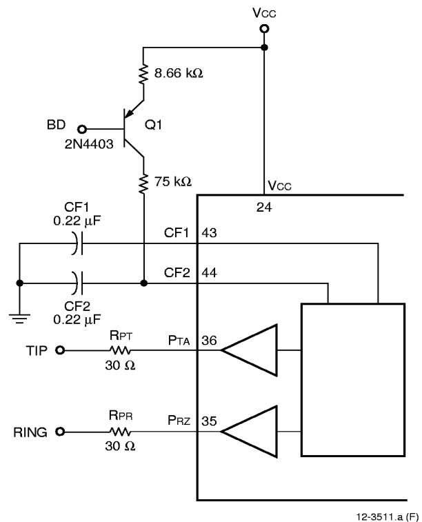
Figure 23. Implementation of a Forward Disconnect State
