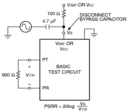
Figure 6. Metallic PSRR
