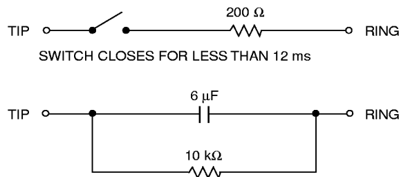
Figure 4. Pretrip Circuit
