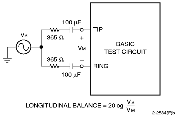
Figure 8. Longitudinal Balance
