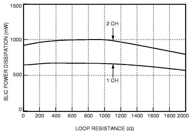
Figure 15. SLIC Power Dissipation vs. Loop Resistance ( V_{BAT} = -48\text{ V} )
