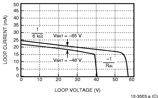
Figure 17. Loop Current vs. Loop Voltage
