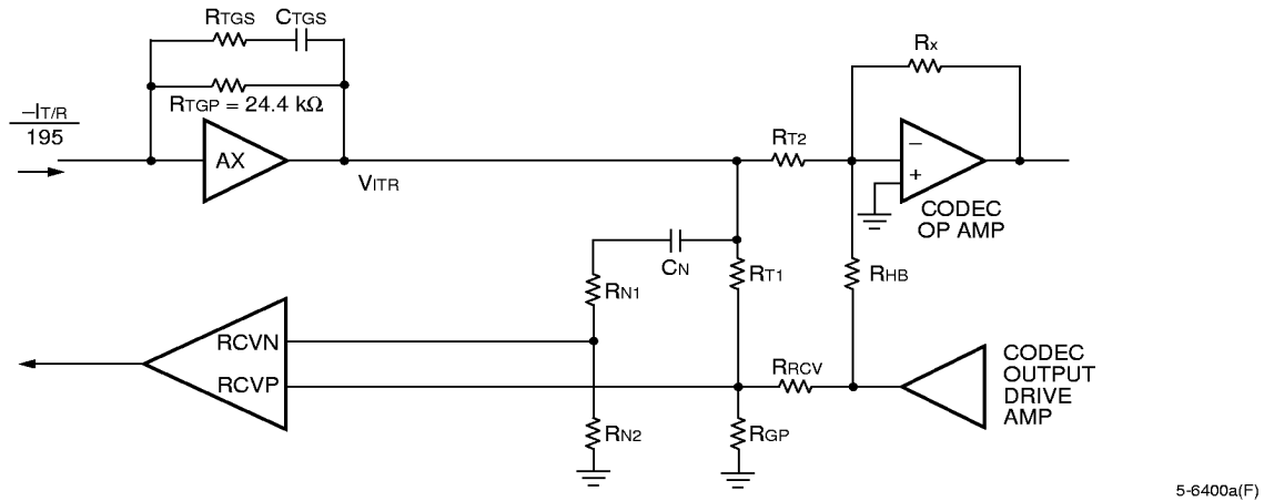
Figure 21. ac Interface Circuit Using First-Generation Codec (Blocking Capacitors Not Shown)
