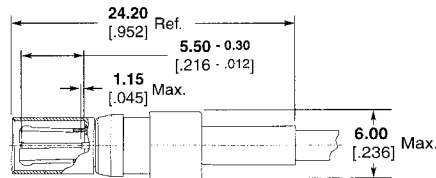
Part Number 148253-1
