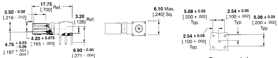
Part Number 1-1393662-2
