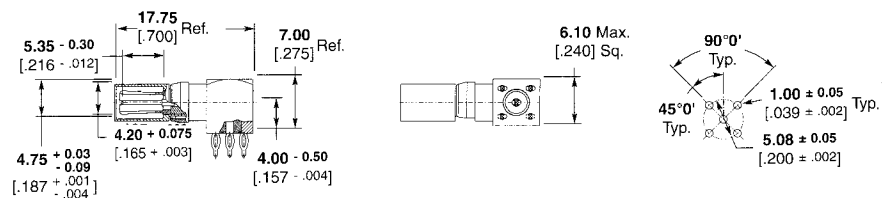
Part Number 148386-1
