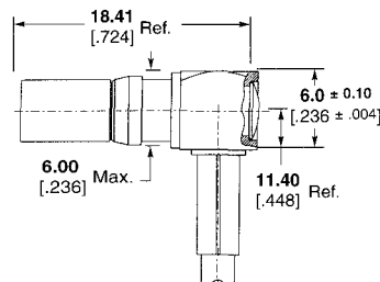
Part Number 148342-1
