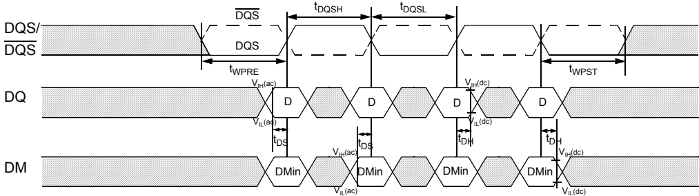
Figure 3. Data Input (Write) Timing
