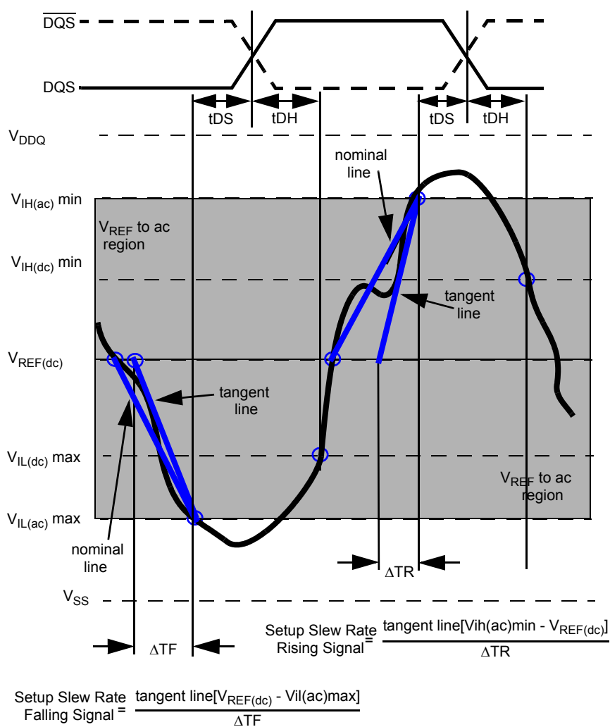
Figure 7. Illustration of tangent line for tDS (differential DQS, DQS)
