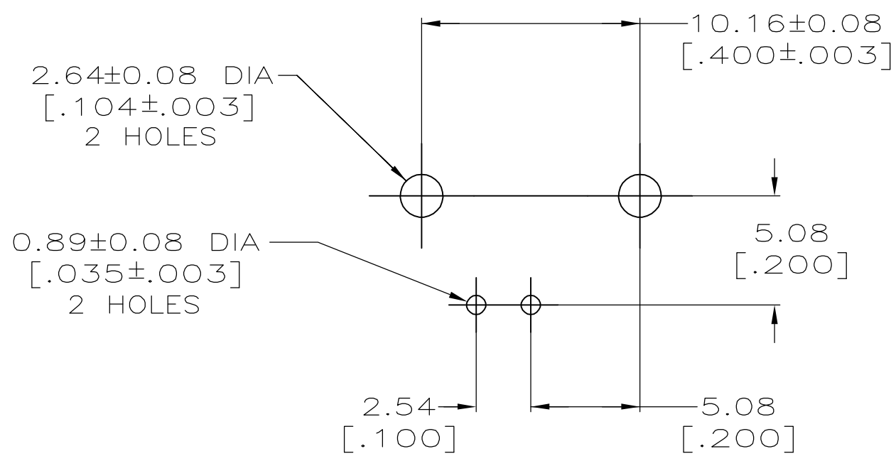
PCB CONFIGURATION
