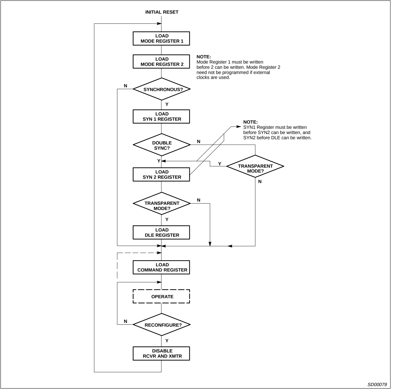
Figure 1. 68661 Initialization Flowchart
