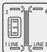
Auxiliary Switch (Note B) Two Pole
