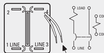
Two Pole (1 pole relay)
