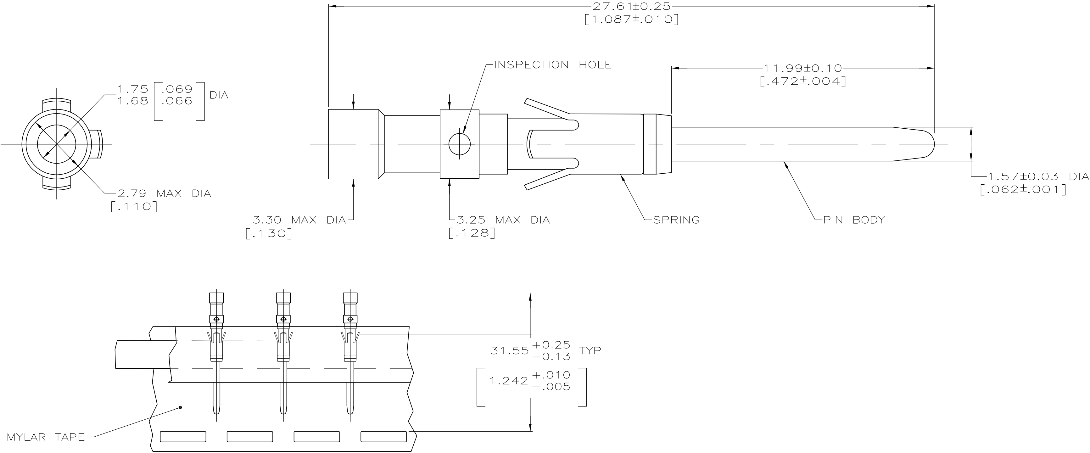
TAPE MTG DETAIL SCALE 2:1
