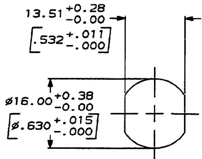
RECOMMENDED PANEL CUTOUT SCALE 2:1
