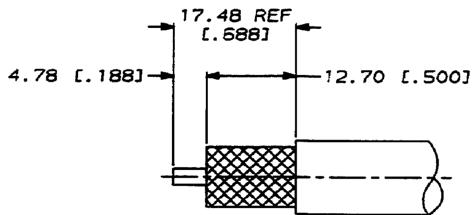
VIEW X RECOMMENDED STRIP LENGTH SCALE 2:1
