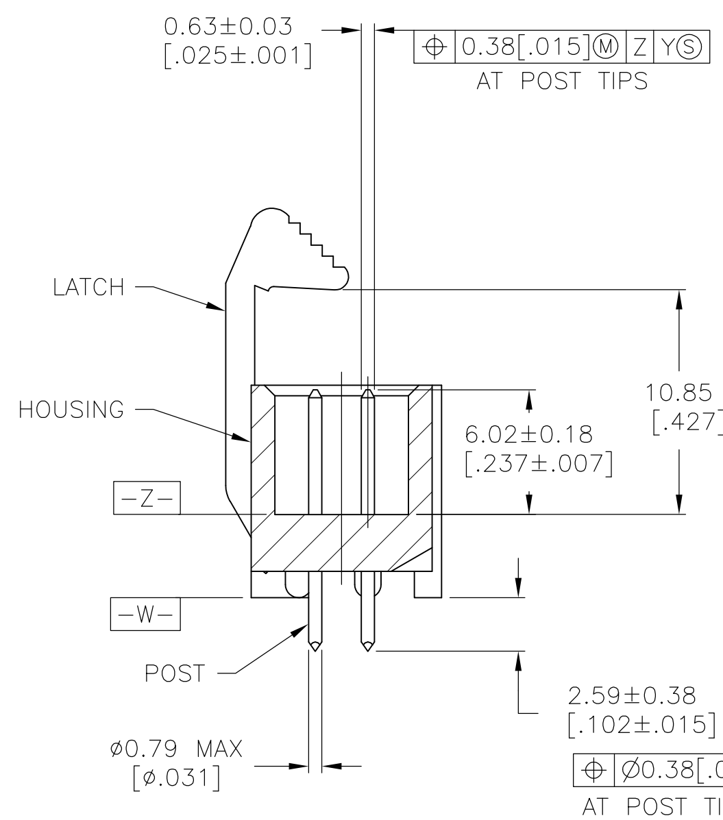
SECTION U-U
