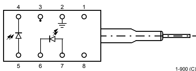
Figure 1. D371-Type Digital Uncooled DFB Laser Module Schematic, Top View
