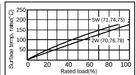
Applied power vs. surface temp.(Example)
