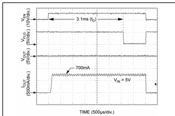
FIGURE 2-25: Enabled into Short-Circuit (MIC2026-1).
