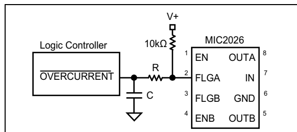
FIGURE 5-2: Transient Filter.
