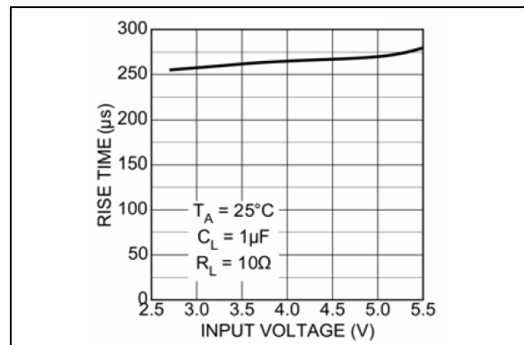
FIGURE 2-12: Rise Time vs. Input Voltage.
