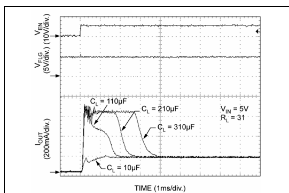
FIGURE 2-26: Inrush Current Response (MIC2026-1).
