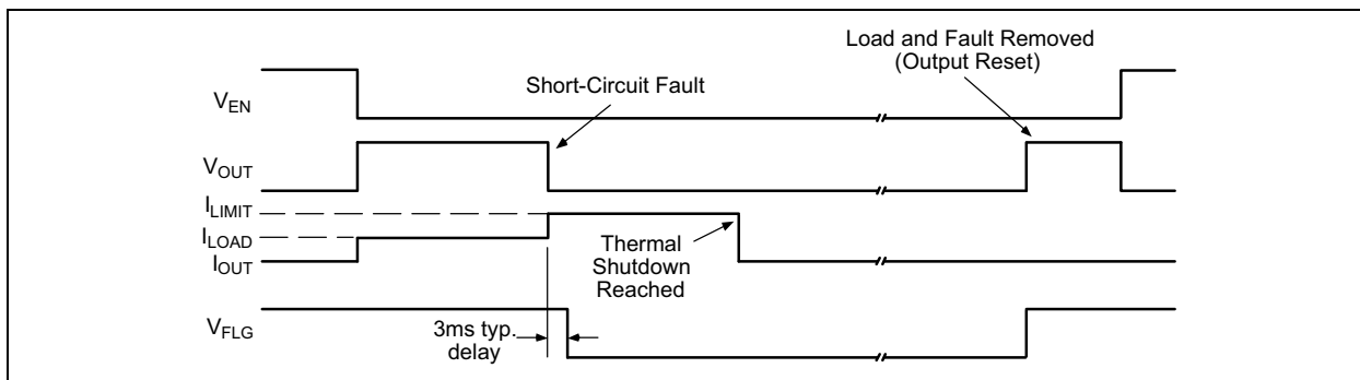
FIGURE 4-1: MIC2076-2 Fault Timing: Output Reset by Removing Load.
