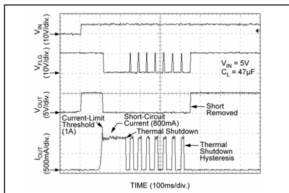
FIGURE 2-27: Current-Limit Response (Ramped Load, MIC2026-1).
