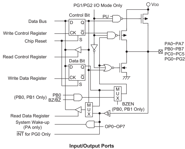
Input/Output Ports
