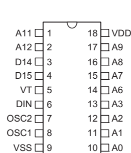
HT692 — 18 DIP-A
