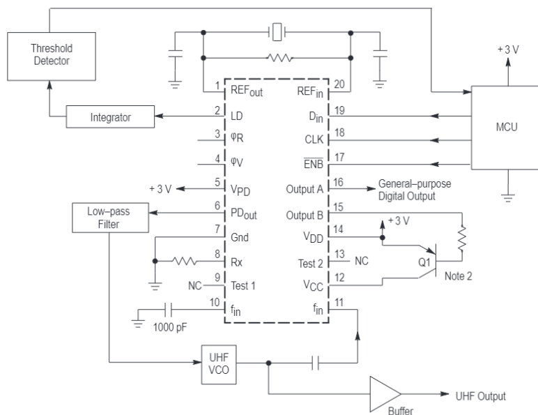
Figure 21. Example Application
