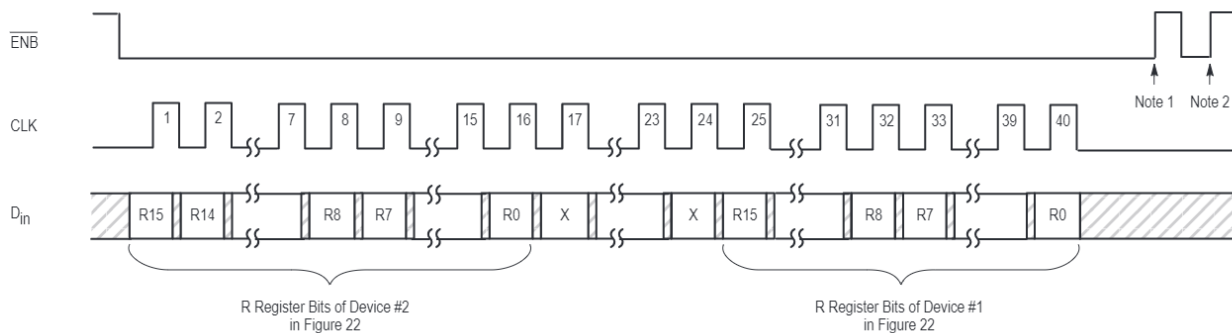
Figure 25. Accessing the R Registers of Two Cascaded MC145193 or MC145202-1 Devices
