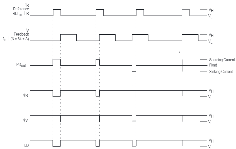
Figure 17. Phase/Frequency Detectors and Lock Detector Output Waveforms
