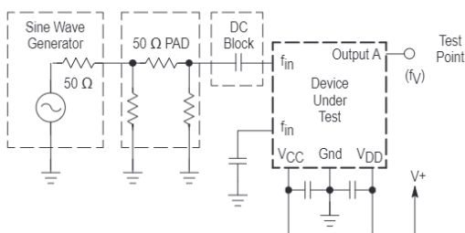
Figure 7. Test Circuit
