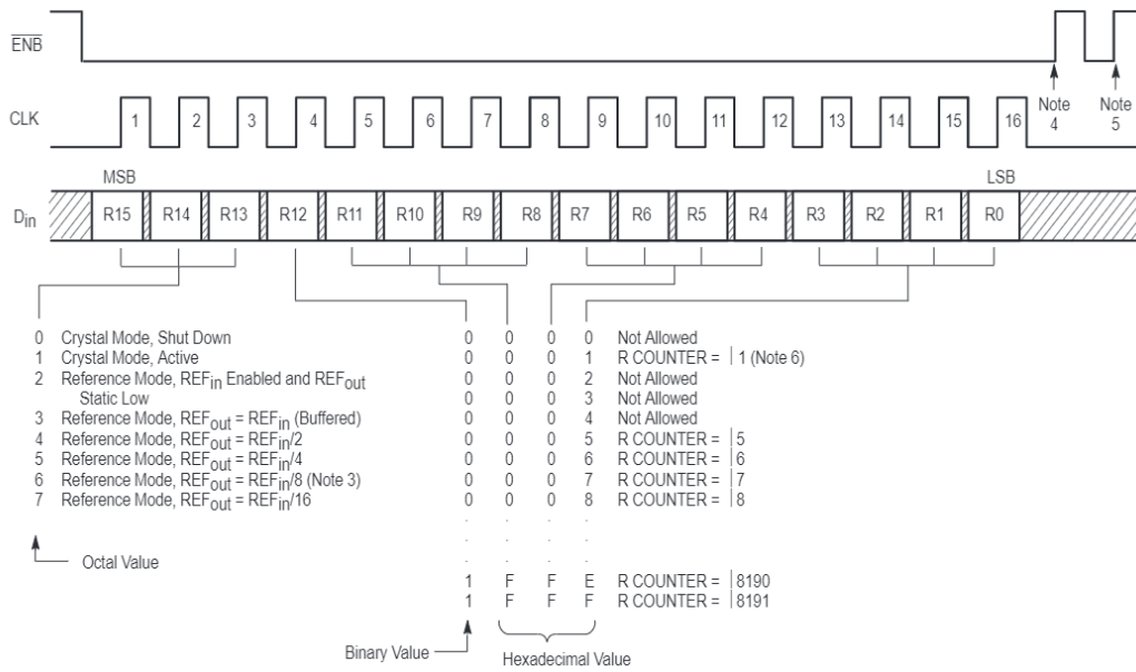
Figure 16. R Register Access and Format (16 Clock Cycles are Used)
