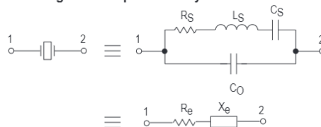
Figure 20. Equivalent Crystal Networks
