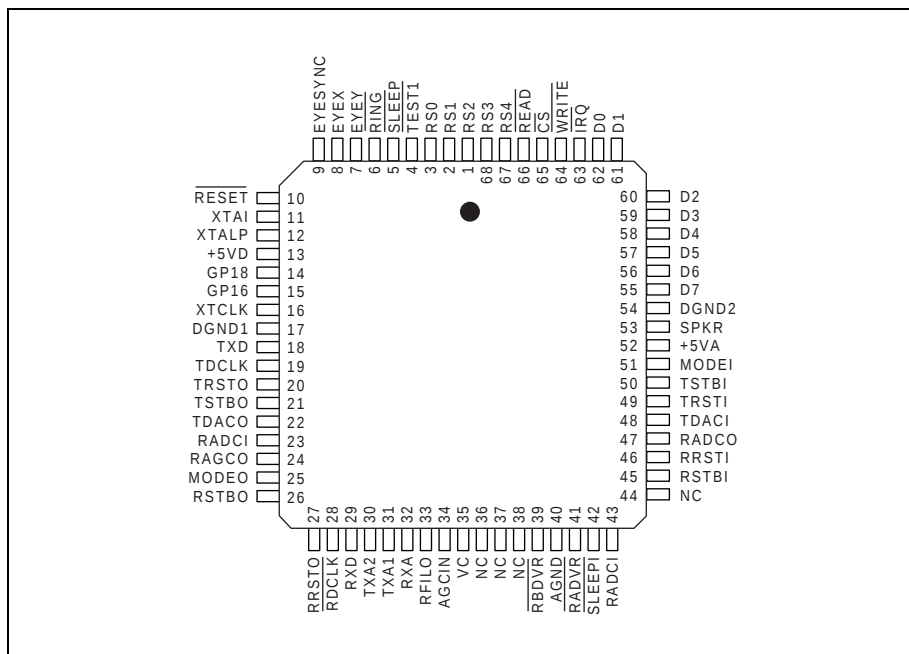
Figure 2-2. RC9623DP Pin Signals
