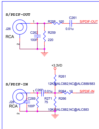
Figure 22. SPDIF Input/Output Connection
