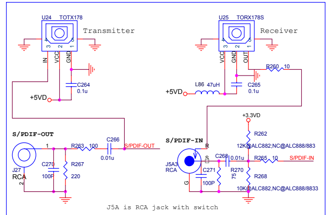
Figure 22. SPDIF Input/Output Connection
