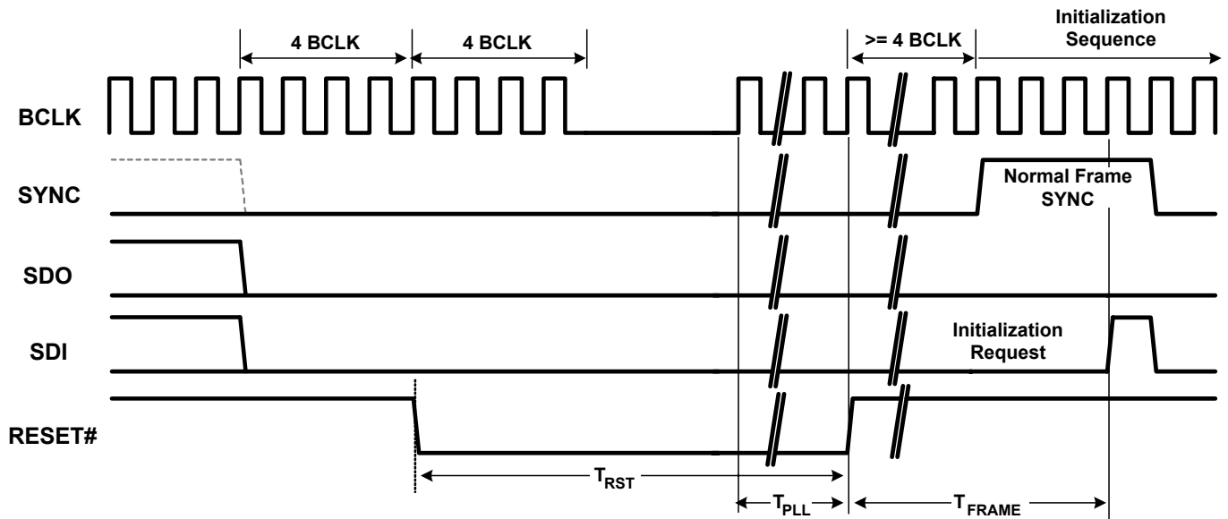
Figure 16. Link Reset and Initialization Timing
