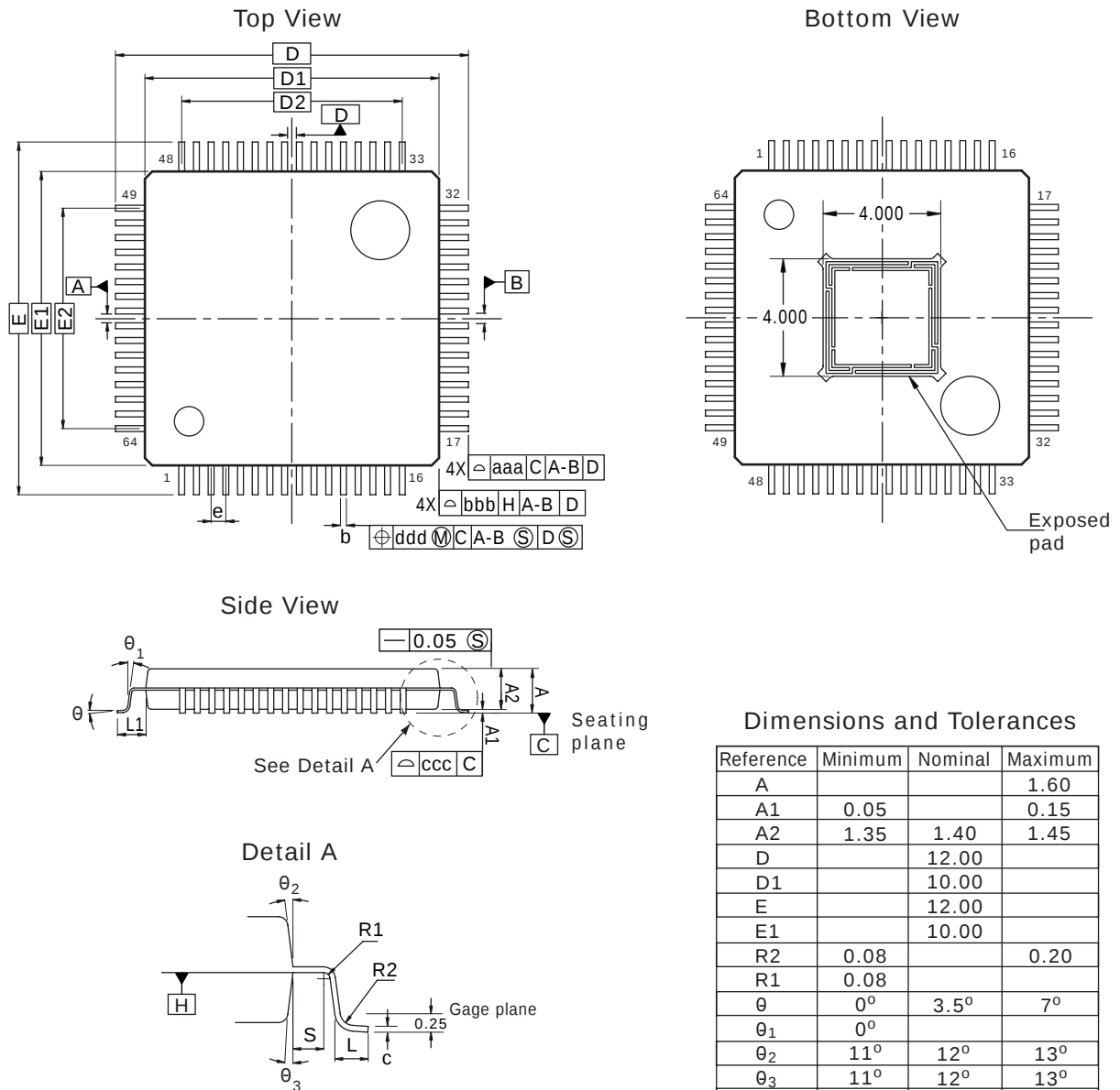
Figure 24. Package Drawing
